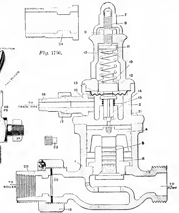
Fig. 1755. Section. AIR-PUMP GOVERNOR.
